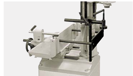
Stop and hold-down set to work in a 180° tilted condition (Stock number 719A-MDA)
