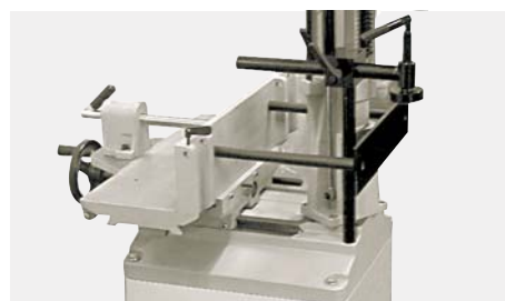
Stop and hold-down set to work in a 180° tilted condition (Stock number 719A-MDA)
